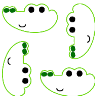
Alligator 55mm Sorted.pes 92.80x92.60 mm; 2,748 stitches 4 thread changes; 4 colors
